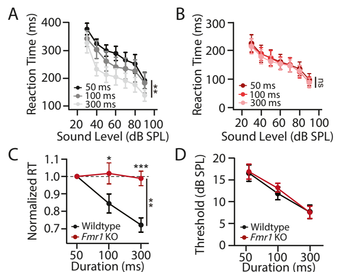
Fig. 2. Disrupted temporal integration of loudness in Fmr1 KO rats. Auditory reaction time-intensity (RT-I) functions measured with broadband noise bursts (BBN) of 50, 100 and 300 ms duration in (A) WT ( \pm SEM, n = 9 ) rats and (B) littermate Fmr1 KO ( \pm SEM, n = 9 ) rats. In WT rats, RTs decreased significantly with intensity ( **p < 0.0025 ) and duration ( ***p < 0.001 ) whereas in Fmr1 KO rats, RTs only decreased significantly with intensity ( *p < 0.0114 ), but not duration ( p = 0.057 ). (C) Mean RTs across intensities (30–90 dB SPL) in WT and KO rats as a function of BBN duration, normalized to mean RTs for 50 ms BBN. RTs in WT rats were modulated by duration to significantly greater extent than Fmr1 KO rats at 100 ms ( **p < 0.01 ) and 300 ms ( ***p < 0.001 ). (D) Threshold of audibility (defined at d' = 1.5 ) plotted as function of BBN duration. Thresholds decreased with duration in both Fmr1 KO and WT rats and there was no significant difference in BBN thresholds across genotypes at any duration.
