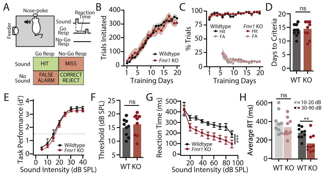
Fig. 1. Psychoacoustic assessment of sound detection thresholds and suprathreshold auditory reaction times in male Fmr1 KO and WT littermate rats. (A) Schematic of operant sound detection apparatus and paradigm. Food-restricted rats were trained to detect broadband noise (BBN) bursts using a Go/No-go paradigm. (B) Fmr1 KO rats (red, n = 9 ) and littermate WT rats (black, n = 9 ) initiated the same number of trials over training days. (C) WT and KO rats generated the same percentage of HITs and false alarms (FAs) over training days. (D) WT and KO rats learned the task to the criteria ( >200 trials/session, >90\% correct, <15\% FA, 5-consecutive days) over the same number of days. (E) Psychometric functions showing mean d' values versus intensity for trained Fmr1 KO and WT rats in response to BBN bursts (1–42 kHz, 50 ms, 0–40 dB SPL, 5 dB steps). (F) No differences in hearing thresholds between KO and WT rats estimated using a criterion of d' = 1.5 (dashed line in E). (G) Reaction time (RT)-intensity functions collected for BBN bursts (1–42 kHz, 50 ms, 10–90 dB SPL, 10 dB steps). RTs were significantly faster in Fmr1 KO animals ( ***p < 0.0001 ). (H) Mean RTs at two lowest intensities (10–20 dB SPL) and five highest intensities (30–90 dB SPL) in WT and Fmr1 KO rats. RTs in WT and KO rats are similar at low intensities, but significantly faster in KO rats at high intensities ( **p < 0.001 ). For this and subsequent figures, data is plotted as mean \pm SEM. Bar graphs represent mean data with overlaid scatter plots of data from each individual animal. (For interpretation of the references to colour in this figure legend, the reader is referred to the web version of this article.)
