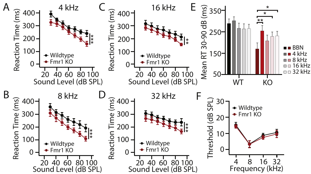
Fig. 4. Loudness growth at different frequencies in WT and Fmr1 KO rats. (A–D) Mean (+/SEM) reaction time-intensity function in WT ( n = 8 ) and KO ( n = 9 ) rats obtained with 300 ms tone bursts at (A) 4 kHz, (B) 8 kHz, (C) 16 kHz and (D) 32 kHz. In both genotypes, RTs varied significantly as a function of sound intensity for all frequencies ( ***p < 0.0001 ). RTs were significantly faster in Fmr1 KO rats than WT rats at 4 kHz ( ***p < 0.0001 ), 8 kHz ( ***p < 0.0001 ), 16 kHz ( **p = 0.0013 ) and 32 kHz ( **p = 0.0002 ). (E) Mean RTs across intensities (30–90 dB SPL) in response to BBN bursts (300 ms) and 4, 8, 16 and 32 kHz tone bursts (300 ms) in Fmr1 KO and WT rats. Among WT rats, mean RT for BBN was not significantly different from mean RT for 4, 8, 16 or 32 kHz. Among Fmr1 KO rats, mean RT for BBN was significantly faster than mean RTs at 4 ( **p < 0.01 ), 16 ( *p < 0.05 ) and 32 kHz ( *p < 0.05 ). (F) Mean (+/SEM) thresholds at 4, 8, 16 and 32 kHz for WT and Fmr1 KO rats. Mean thresholds varied significantly with frequency ( ***p < 0.0001 ), but thresholds were not significantly different across genotypes at any frequency.
