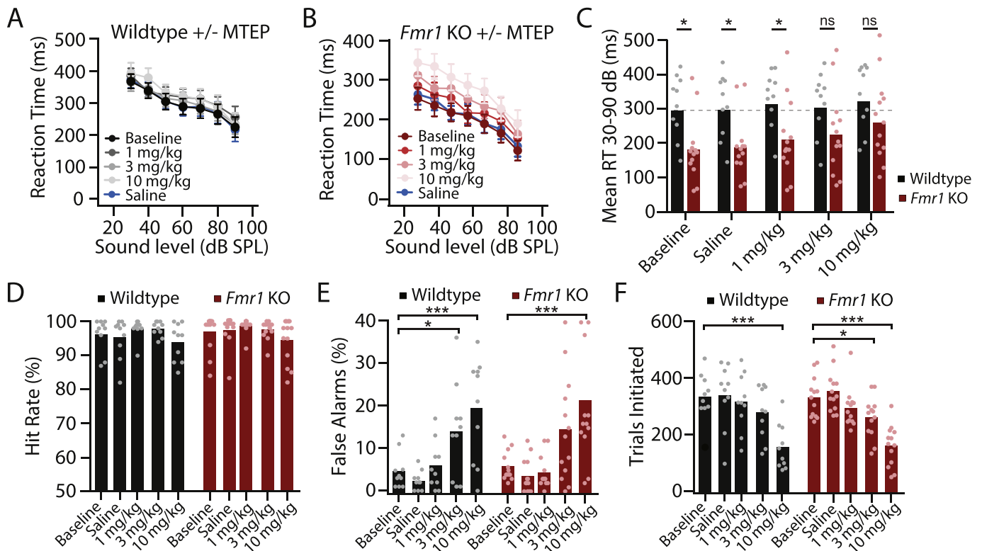
Fig. 5. Inhibition of mGlu5 dose-dependently increases RTs in Fmr1 KO but not WT rats. (A) Mean ( \pm SEM, n = 10 ) reaction time-intensity (RT-I) functions from WT rats treated with different doses of the selective mGlu5 negative allosteric modulator MTEP or saline versus baseline control. Analysis of the RT-I functions revealed a significant effect of intensity ( ***p < 0.0001 ) and treatment ( *p < 0.025 ); however, RTs obtained with MTEP treatments were not significantly different from baseline or saline control conditions. (B) Mean ( \pm SEM, n = 12 ) RT-I functions from Fmr1 KO rats treated with different doses of MTEP or saline versus baseline control. Analysis of the RT-I functions revealed a significant effect of intensity ( ***p < 0.0001 ) and treatment ( ***p < 0.0001 ) and RT-I functions were significantly different from baseline and saline control conditions when treated with 3 mg/kg ( **p = 0.004 ) or 10 mg/kg ( ***p < 0.001 ) MTEP. (C) Mean RTs from 30 to 90 dB SPL in WT and Fmr1 KO rats for baseline, saline, and 1, 3, and 10 mg/kg MTEP conditions. RTs were significantly faster in Fmr1 KO rats compared WT rats for the baseline, saline control, and 1 mg/kg MTEP conditions ( *p < 0.05 ). Mean values for WT and Fmr1 KO rats were not significantly different from one another for the 3 and 10 mg/kg MTEP treatments ( p > 0.05 ). (D) Mean percent correct responses did not differ across experimental conditions in WT ( p = 0.107 ) or Fmr1 KO rats ( p = 0.102 ). (E) Mean percent false alarms in WT and Fmr1 KO rats varied significantly across treatment ( ***p < 0.0001 ) but there was no significant effect of genotype ( p = 0.703 ). False alarm rates were significantly greater with 3 mg/kg ( *p < 0.05 ) and 10 mg/kg ( ***p < 0.001 ) MTEP treatment in WT animals and were significantly greater in KO animals at 10 mg/kg MTEP treatment ( ***p < 0.001 ) compared to baseline. (F) Mean trials initiated in WT rats and Fmr1 KO rats varied significantly across treatment ( ***p < 0.0001 ) but there was no significant effect of genotype ( p = 0.8496 ). Trial number was significantly decreased with 10 mg/kg ( ***p < 0.001 ) MTEP treatment in WT animals and was significantly decreased in KO animals with 3 mg/kg ( *p < 0.05 ) and 10 mg/kg ( ***p < 0.001 ) MTEP treatment compared to baseline. Bar graphs represent mean data with overlaid scatter plots of data from each individual animal.
