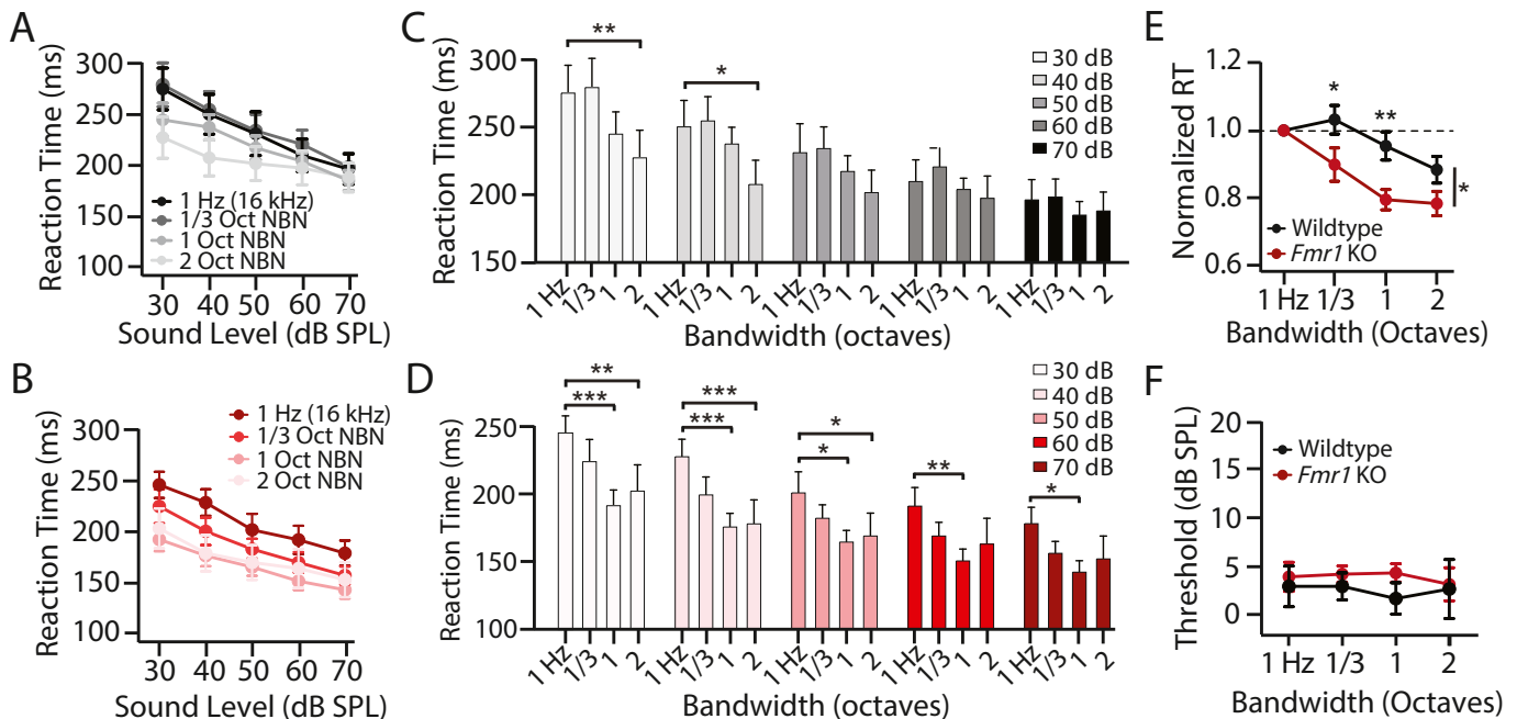
Fig. 3. Altered spectral integration of loudness in Fmr1 KO rats. (A–B) Mean (+/-SEM) reaction time-intensity (RT-I) functions in WT ( n = 8 ) and littermate Fmr1 KO ( n = 8 ) rats. Stimuli were 300 ms tone bursts (16 kHz, 1 Hz nominal bandwidth) and 300 ms narrow band noise (NBN) bursts centered at 16 kHz with bandwidths of 1/3, 1, or 2 octaves (Oct) from 30 to 70 dB SPL in 10 dB steps. (A) Mean (+/-SEM) RT-I functions in WT animals. RTs decreased significantly with intensity ( ***p < 0.0001 ) and bandwidth ( *p = 0.016 ) and there was a significant bandwidth-intensity interaction ( *p = 0.012 ). (B) Mean (+/-SEM) RT-I functions in Fmr1 KO animals. RTs decreased significantly with intensity ( ***p < 0.0001 ) and bandwidth ( ***p = 0.004 ) and the interaction between bandwidth and intensity was not significant. (C) Mean RTs (+SEM) at each bandwidth (1 Hz, 1/3, 1, and 2 Oct) and each intensity (30–70 dB SPL) in WT animals. RTs at 1 Hz (16 kHz) were significantly slower from 2 Oct NBN at 30 and 40 dB SPL only ( *p < 0.05 ). (D) Mean (+SEM) RTs at each bandwidth (1 Hz, 1/3, 1, and 2 Oct) and each intensity (30–70 dB SPL) in Fmr1 KO animals. Significant differences in RT between 1 Hz (16 kHz) and 1 and/or 2 Oct NBN at all intensities ( *p < 0.05 , **p < 0.01 , ***p < 0.001 ). (E) Mean RTs from 30 to 70 dB SPL in WT and KO rats as a function of bandwidth, normalized to 1 Hz. The effect of bandwidth on RTs was significantly greater for Fmr1 KO versus WT animals for 1/3 ( *p < 0.05 ) and 1 ( *p < 0.01 ) octave band noise. (F) Mean (+/-SEM) thresholds as a function of bandwidth in Fmr1 KO and WT rats. Thresholds (defined at d' = 1.5 ) were not affected by bandwidth and there was no significant difference in thresholds across genotypes at any bandwidth.
