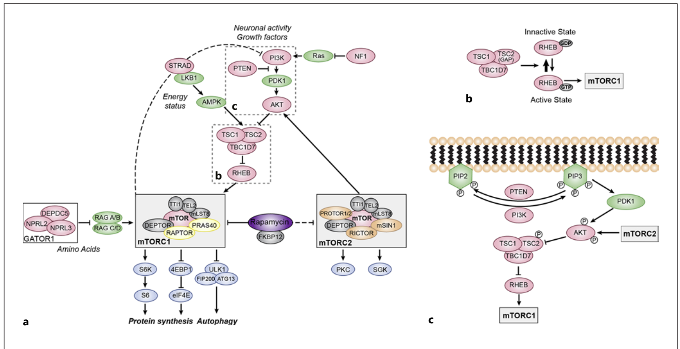
Fig. 1. Mutations in regulators of mTOR signaling cause mTORopathies. a mTOR is a protein kinase found in two distinct multiprotein complexes, mTORC1 and mTORC2, which are composed of shared and unique protein components. Several upstream regulators collectively work to control the activity of the two complexes in response to various stimuli including growth factors and nutrients. Mutations in genes that encode for mTOR regulators (denoted in pink) result in neurodevelopmental disorders, collectively termed mTORopathies (see Table 1). Current treatments for mTORopathies include rapalogs, which are derivatives of rapamycin that suppress mTORC1 activity and indirectly inhibit mTORC2 signaling when administered chronically. b The TSC complex functions as a GAP for the small GTPase RHEB, which is a direct activator of mTORC1. c PI3K converts PIP2 into PIP3 via phospho-
